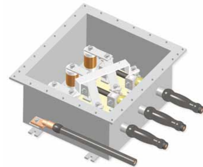
Buried Type : Link Box for cross bonding(3-1Way)
